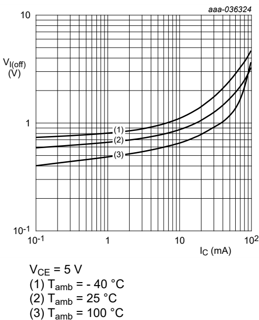
Fig. 5. TR1 (NPN): Off-state input voltage as a function of collector current; typical values
