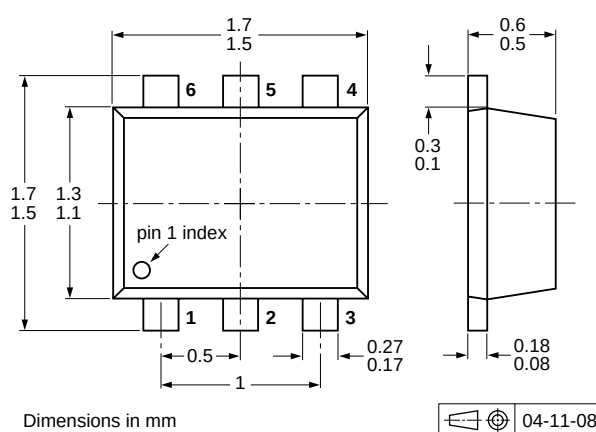
Fig 4. Package outline SOT666
