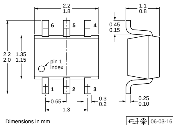
Fig 3. Package outline SOT363 (SC-88)
