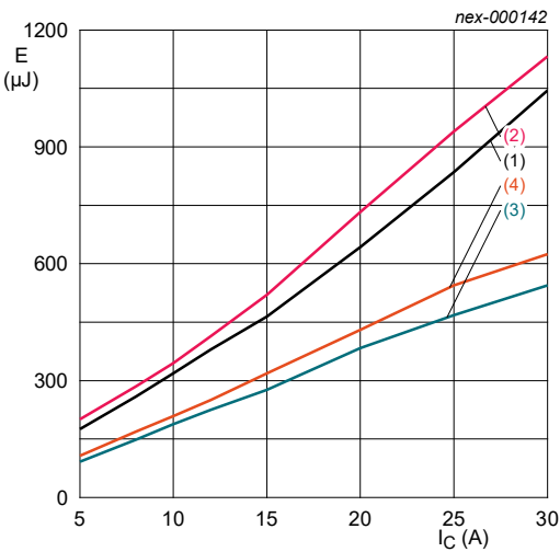
V_{GE} = \pm 15\text{ V}; V_{CC} = 400\text{ V} R_{G(on)} = 15\ \Omega; R_{G(off)} = 36\ \Omega • (1) E_{on}, T_{vj} = 125\text{ }^{\circ}\text{C} • (2) E_{on}, T_{vj} = 175\text{ }^{\circ}\text{C} • (3) E_{off}, T_{vj} = 125\text{ }^{\circ}\text{C} • (4) E_{off}, T_{vj} = 175\text{ }^{\circ}\text{C}
