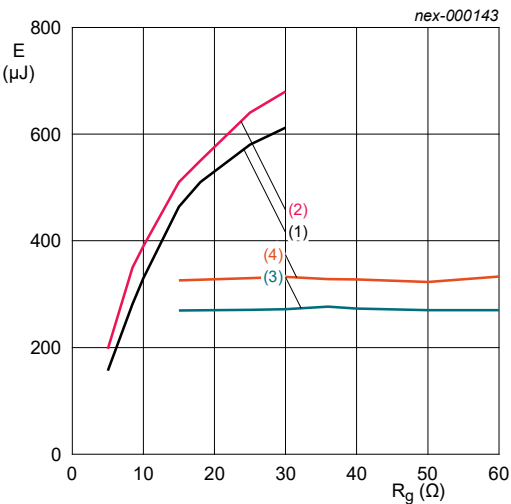
V_{GE} = \pm 15\text{ V}; V_{CC} = 400\text{ V}; I_C = 15\text{ A} • (1) E_{on}, T_{vj} = 125\text{ }^{\circ}\text{C} • (2) E_{on}, T_{vj} = 175\text{ }^{\circ}\text{C} • (3) E_{off}, T_{vj} = 125\text{ }^{\circ}\text{C} • (4) E_{off}, T_{vj} = 175\text{ }^{\circ}\text{C}
