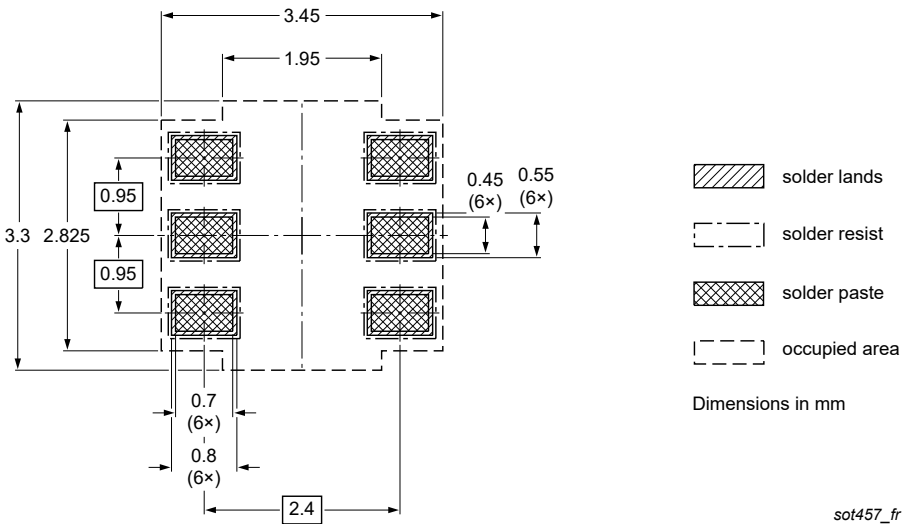
Fig. 19. Reflow soldering footprint for TSOP6 (SOT457)
