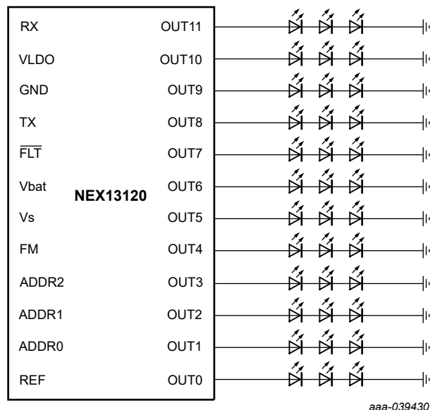
Fig. 1. Typical application
