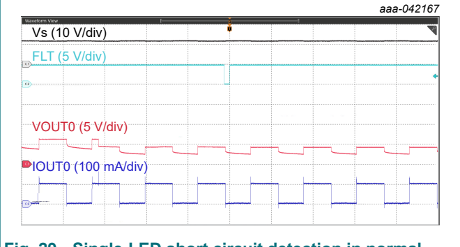
Fig. 29. Single-LED short circuit detection in normal mode
