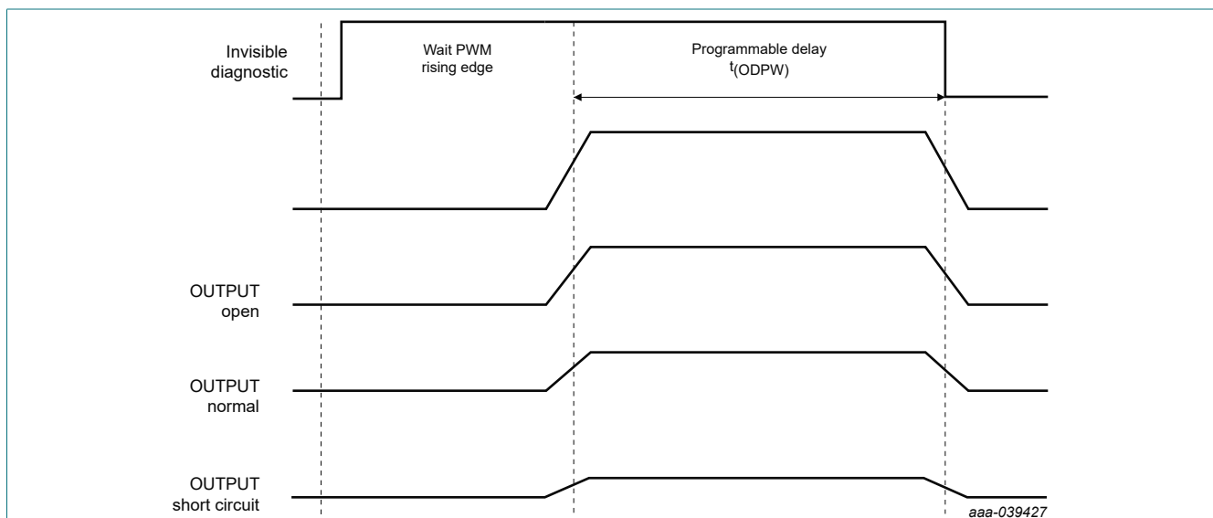
Fig. 36. Programmable invisible diagnostics timing sequence
