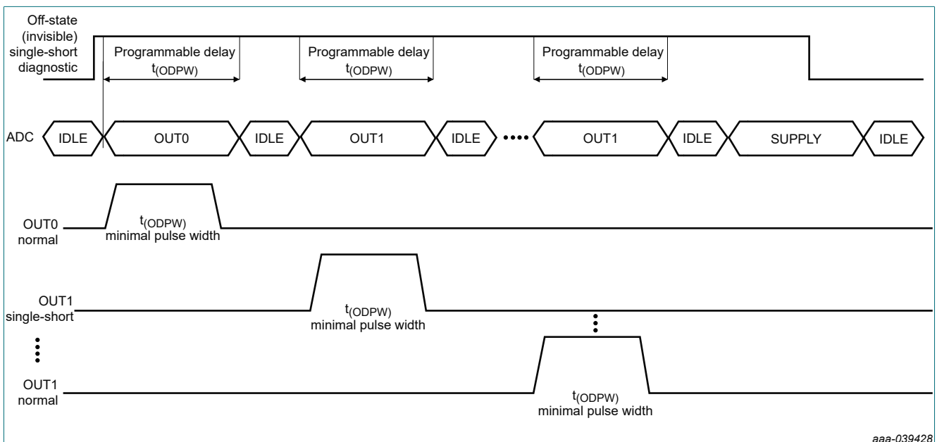
Fig. 37. Single-LED short-circuit OFF-state timing sequence
