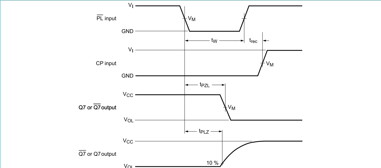
Fig. 12. The parallel load ( \overline{PL} ) pulse width, the parallel load to output ( Q7 or \overline{Q7} ) propagation delays, the parallel load to clock ( CP ) recovery times
